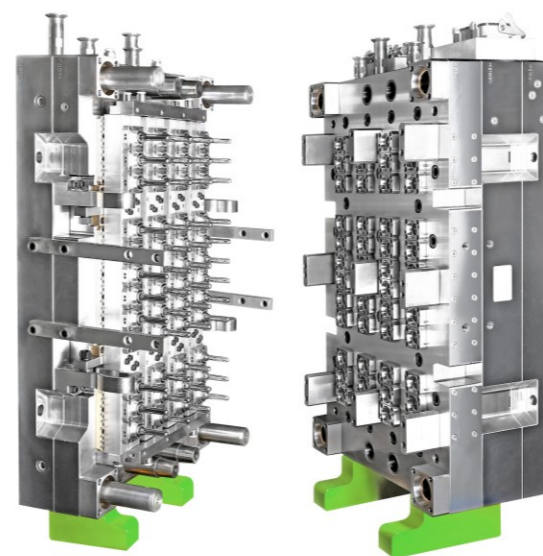
48 cavities
