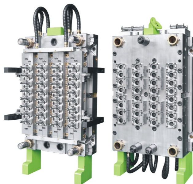
32 cavities
